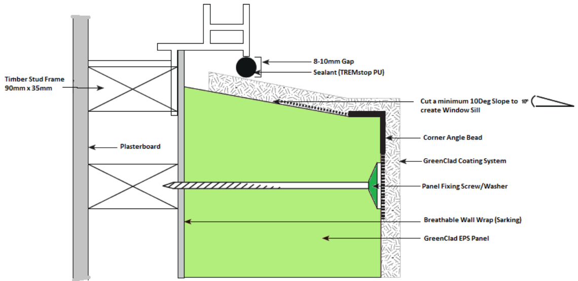
Typical Aluminium Frame Window Sill Detail
