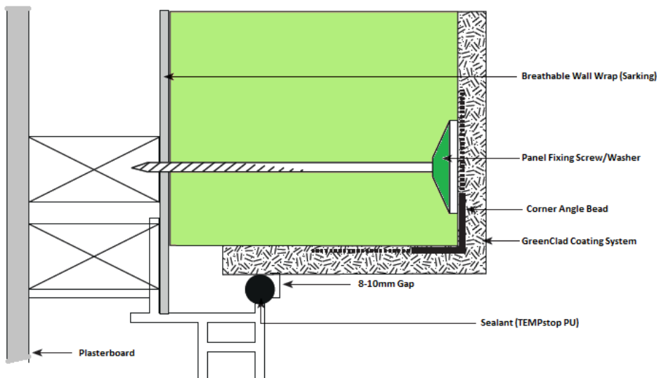
Typical Aluminium Frame Jamb Detail
