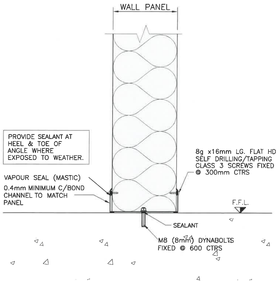
PARTITION WALL EXT'L WALL BASE DETAIL
