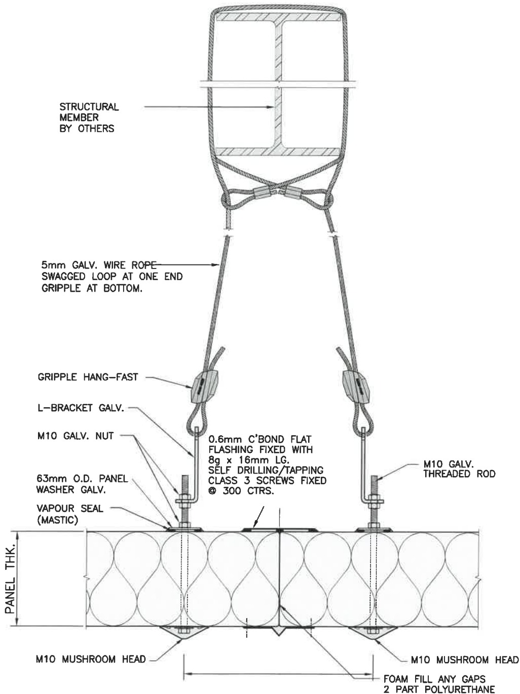
MAIN CEILING SUSPENSION
