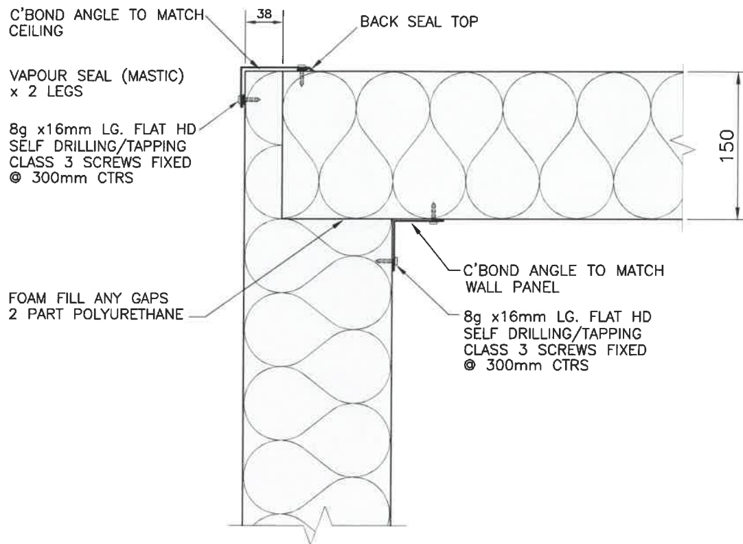
WALL TO CEILING DETAIL
