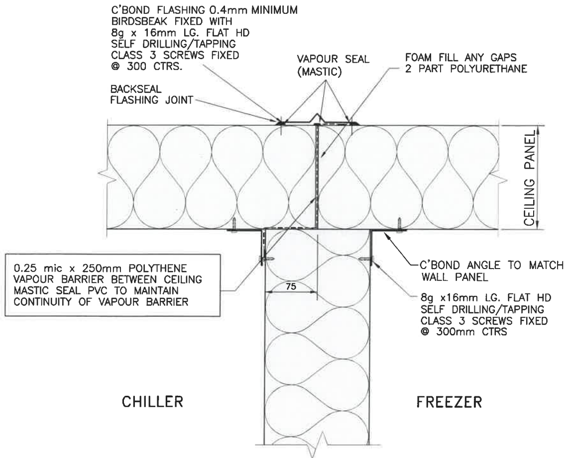
CEILING CONNECTION CHILLER TO FREEZER
