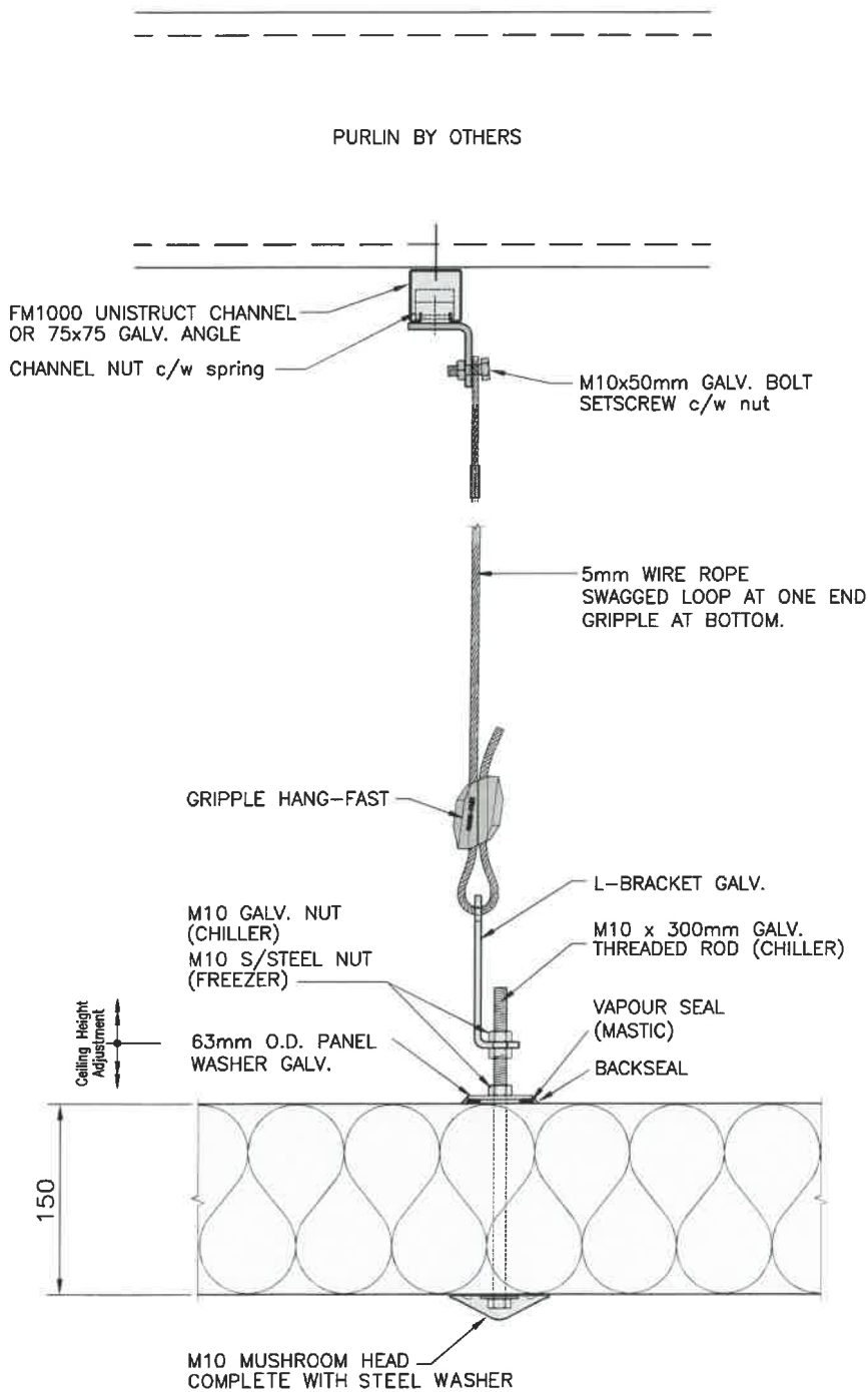
INTERMEDIATE CEILING SUSPENSION
